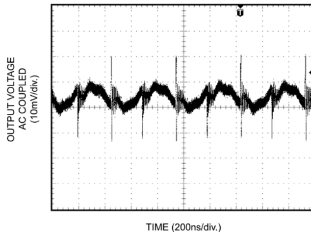
Output Ripple
