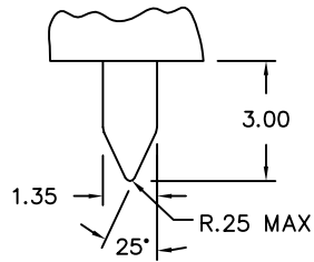
VIEW E, NOTE 8 SCALE 2:1
