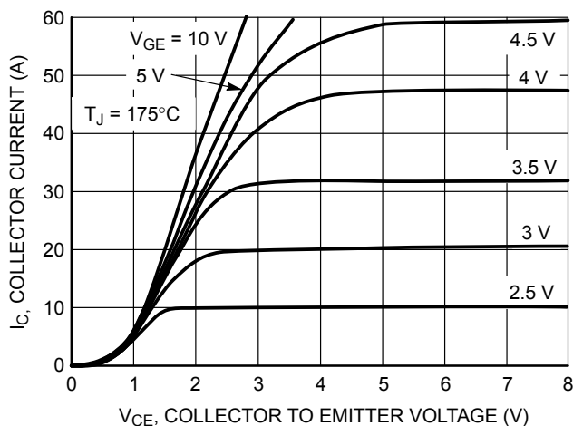
Figure 4. Collector Current vs. Collector-to-Emitter Voltage
