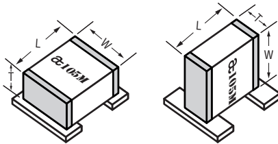
Horizontal Electrode Orientation Vertical Electrode Orientation
