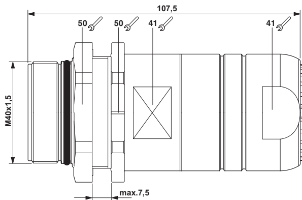
Dimensioned drawing
