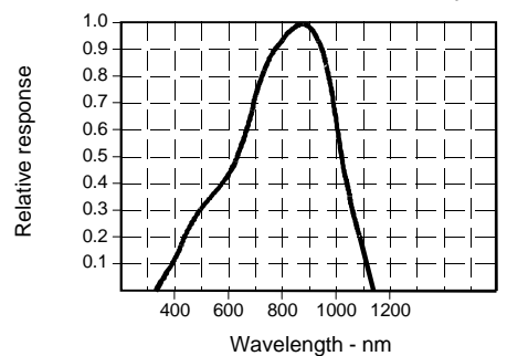
Fig. 4 Spectral Responsivity
