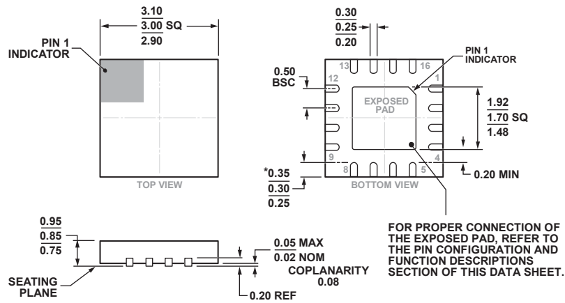
Figure 20. 16-Lead Lead Frame Chip Scale Package [LFCSP_WQ] 3 mm × 3 mm Body, Very Very Thin Quad (CP-16-38)
