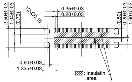
Recommended metal mask pattern Metal mask thickness: When 100 \mu m (Terminal opening ratio: 70%) (Metal-part opening ratio: 46%)
