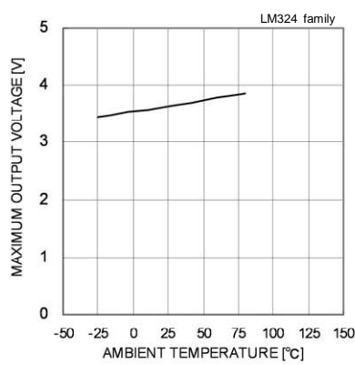
Fig. 29 Maximum Output Voltage - Ambient Temperature ( V_{CC}=5[V], R_L=2[k\Omega] )
