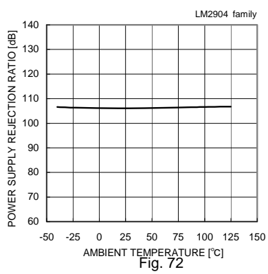
Fig. 72 Power Supply Rejection Ratio – Ambient Temperature
