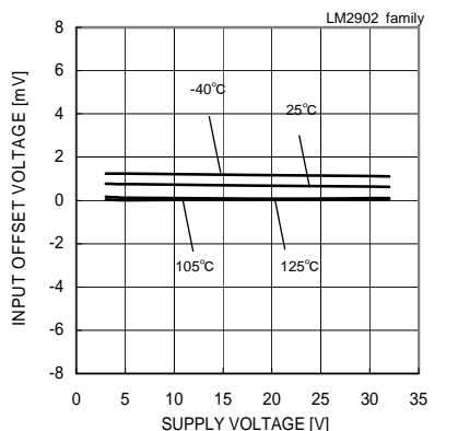
Fig. 84 Input Offset Voltage - Supply Voltage ( V_{icm}=0[V] , V_{OUT}=1.4[V] )
