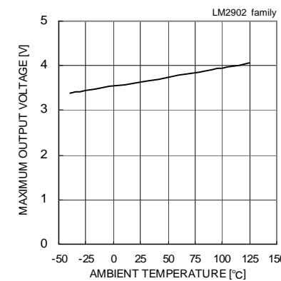
Fig. 77 Maximum Output Voltage - Ambient Temperature ( V_{CC}=5[V] , R_L=2[k\Omega] )
