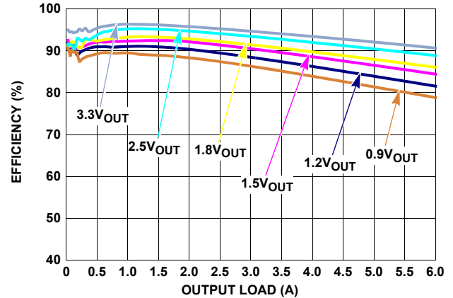
FIGURE 11. EFFICIENCY vs LOAD (2MHz 5VIN PFM)
