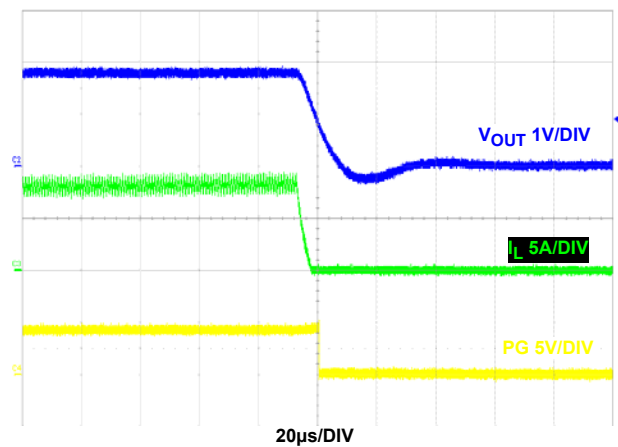
FIGURE 48. OVERCURRENT PROTECTION
