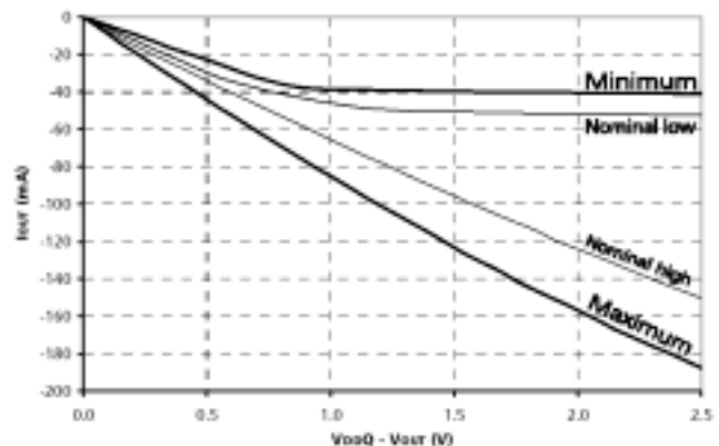
Figure 8: Pull-Up Characteristics
