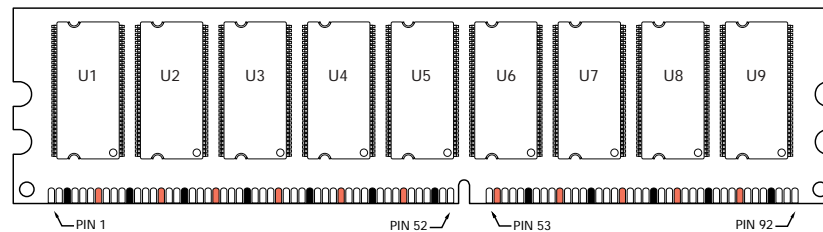
Figure 2: Pin Locations: 184-PIN DIMM
