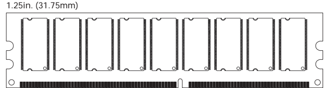
Figure 1: 184-Pin DIMM (MO-206)
