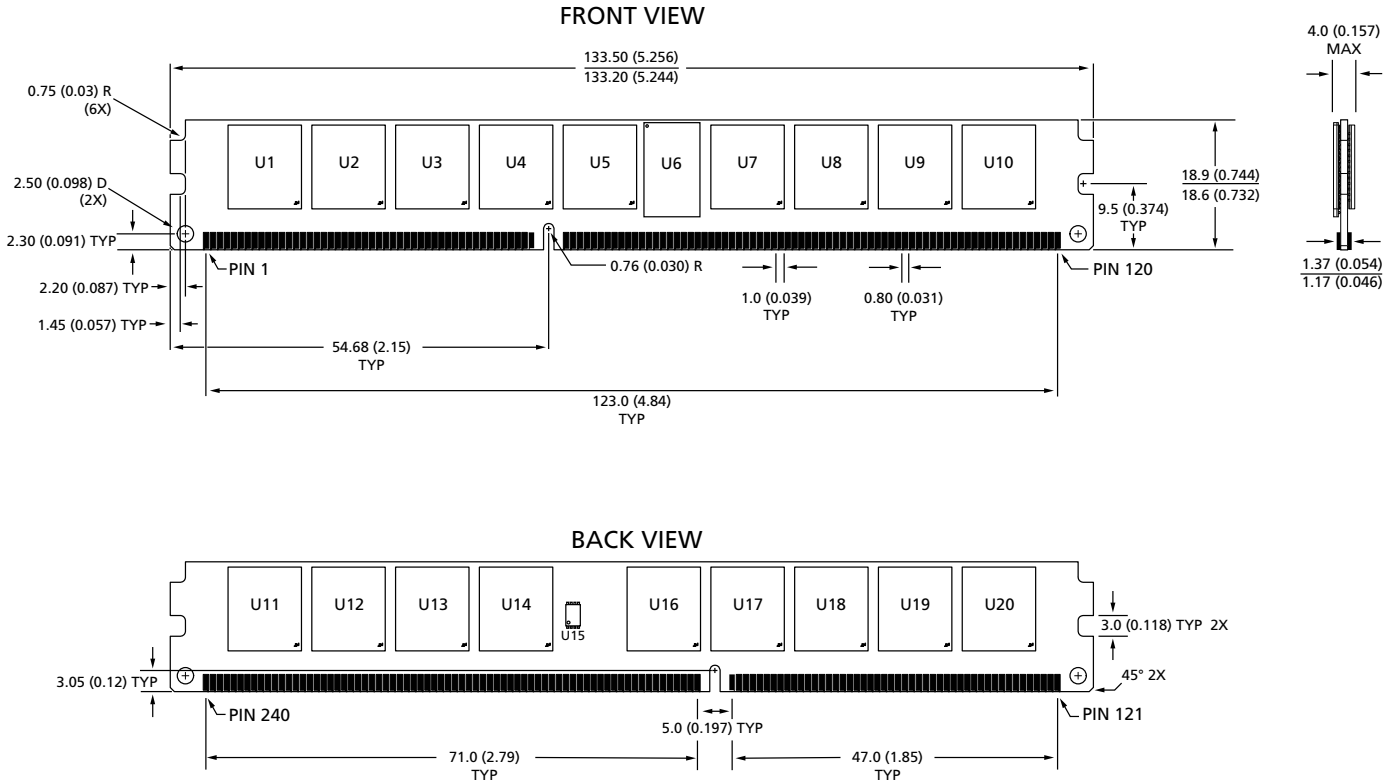
Figure 3: 240-Pin DDR3 RDIMM
