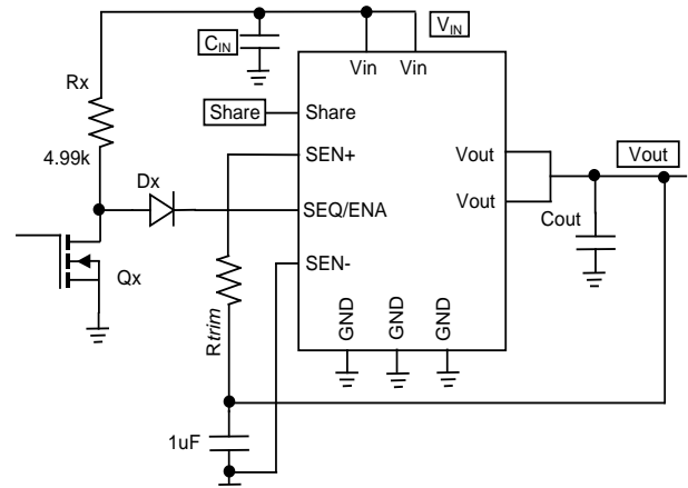
Figure 24. Application Schematic
