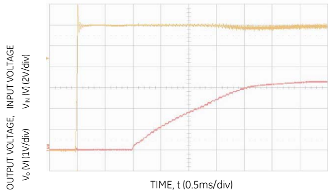
Figure 11. Typical Start-Up with application of V_{in} ( V_o = 3.3V dc).
