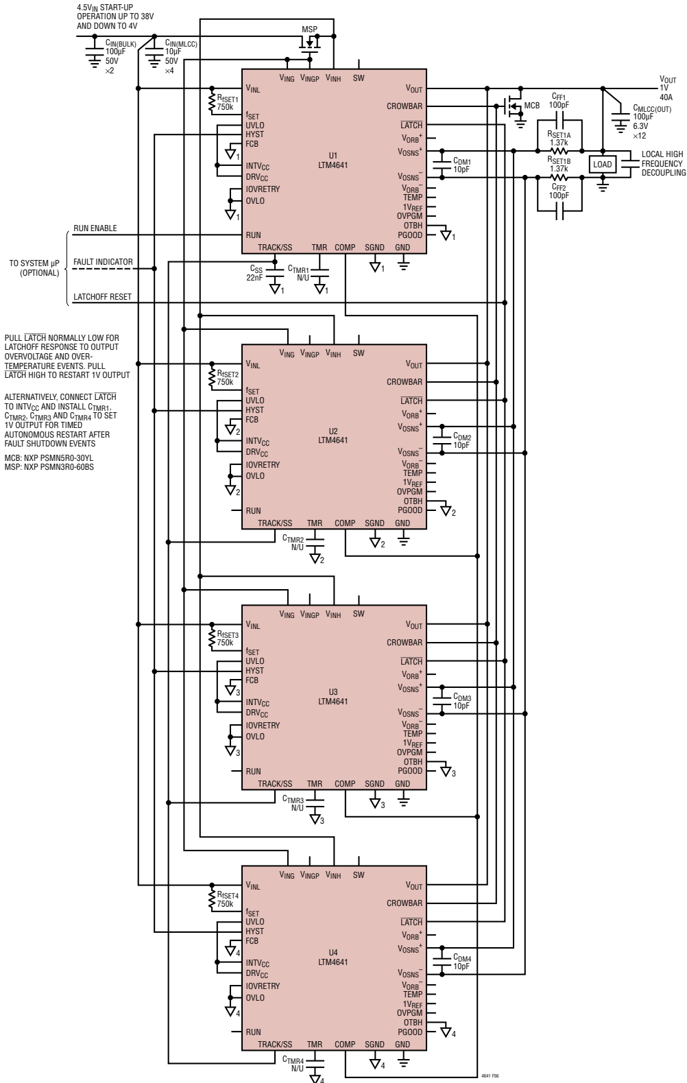
U1, U2, U3 AND U4 SGND (▽ 1 , ▽ 2 , ▽ 3 , ▽ 4 ) CONNECT TO GND INTERNAL TO THEIR RESPECTIVE MODULES. KEEP MODULE SGND ROUTES/PLANES SEPARATE FROM OTHER MODULES AND FROM GND ON MOTHERBOARD
