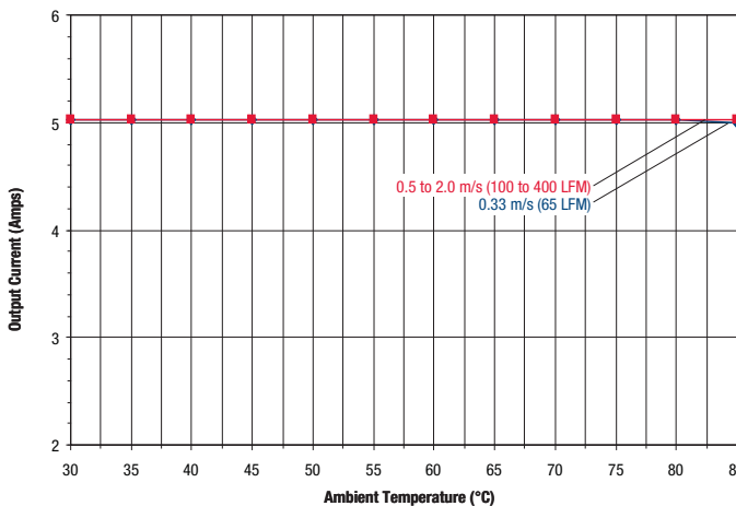
Maximum Current Temperature Derating @ sea level (Vin = 48V, air flow from Pin 1 to Pin 3 on PCB, no baseplate)
