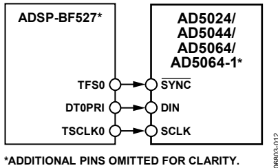
*ADDITIONAL PINS OMITTED FOR CLARITY. 06803-012 Figure 52. AD5024/AD5044/AD5064/AD5064-1 to Blackfin ADSP-BF527 Interface
