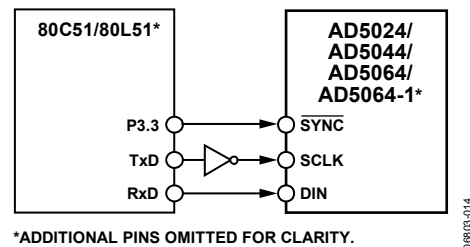
*ADDITIONAL PINS OMITTED FOR CLARITY. 06803-014 Figure 54. AD5024/AD5044/AD5064/AD5064-1 to 80C51/80L51 Interface
