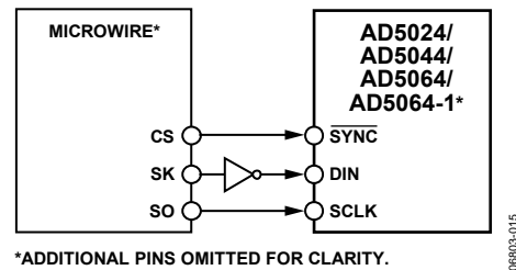
*ADDITIONAL PINS OMITTED FOR CLARITY. 06803-015 Figure 55. AD5024/AD5044/AD5064/AD5064-1 to MICROWIRE Interface
