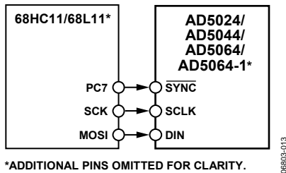
*ADDITIONAL PINS OMITTED FOR CLARITY. 06803-013 Figure 53. AD5024/AD5044/AD5064/AD5064-1 to 68HC11/68L11 Interface
