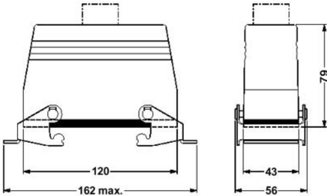
Dimensioned drawing
