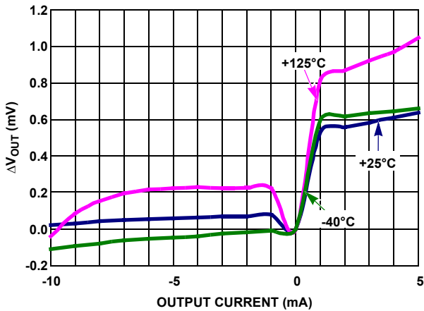
FIGURE 5. LOAD REGULATION
