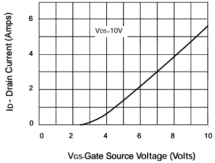
Transfer Characteristics
