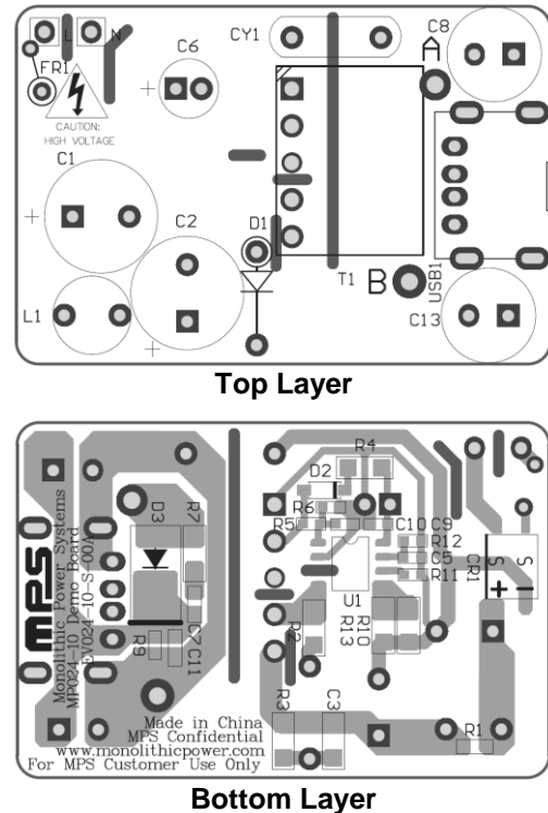
Figure 15: Recommended Layout
