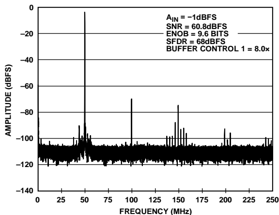
Figure 88. Single-Tone FFT with f_{IN} = 1950.3 MHz
