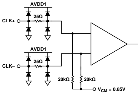
Figure 105. Clock Inputs
