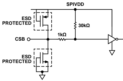
Figure 110. CSB Input
