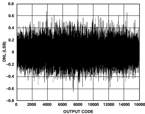
Figure 100. DNL, f_{IN} = 15 MHz
