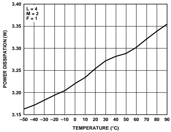
Figure 53. Power Dissipation vs. Temperature
