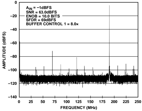
Figure 86. Single-Tone FFT with f_{IN} = 1310.3 MHz
