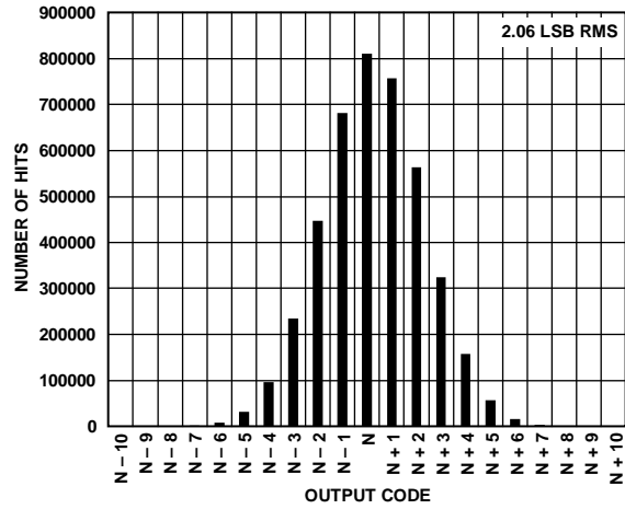
Figure 101. Input-Referred Noise Histogram
