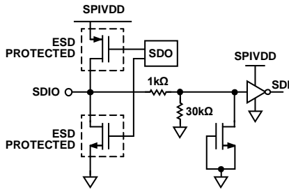
Figure 111. SDIO Input
