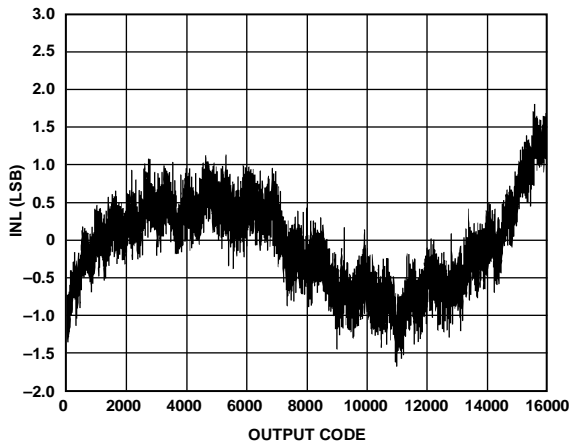
Figure 99. INL, f_{IN} = 10.3 MHz
