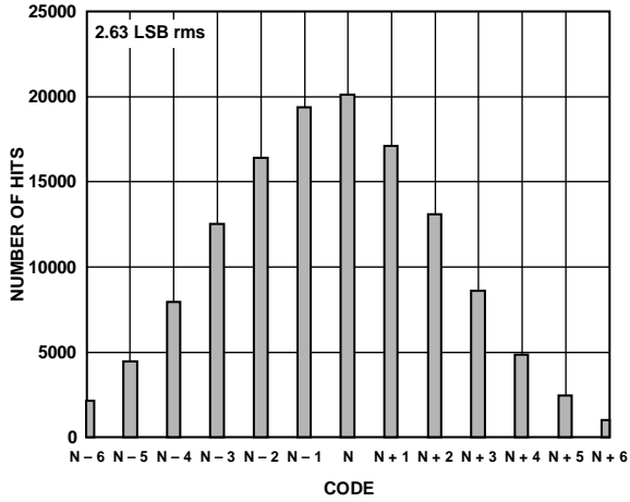
Figure 52. Input-Referred Noise Histogram
