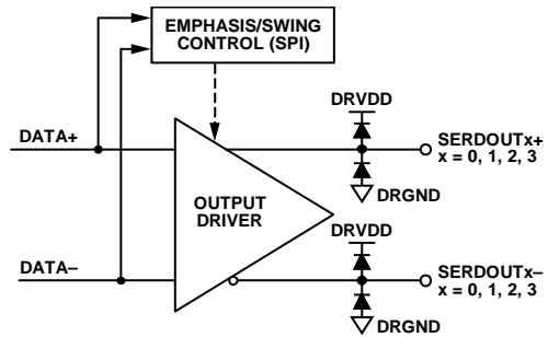
Figure 107. Digital Outputs
