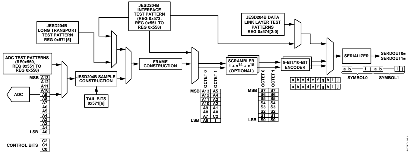
Figure 156. ADC Output Data Path Showing Data Framing
