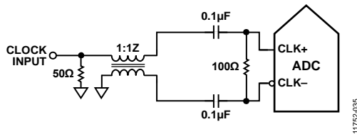
Figure 134. Transformer-Coupled Differential Clock
