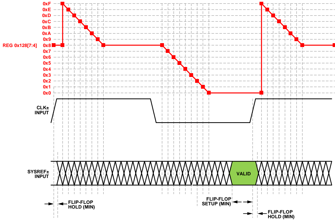
Figure 173. SYSREF± Hold Detector
