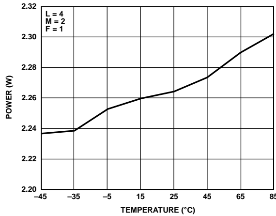
Figure 102. Power Dissipation vs. Temperature
