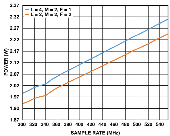
Figure 103. Power Dissipation vs. f_s
