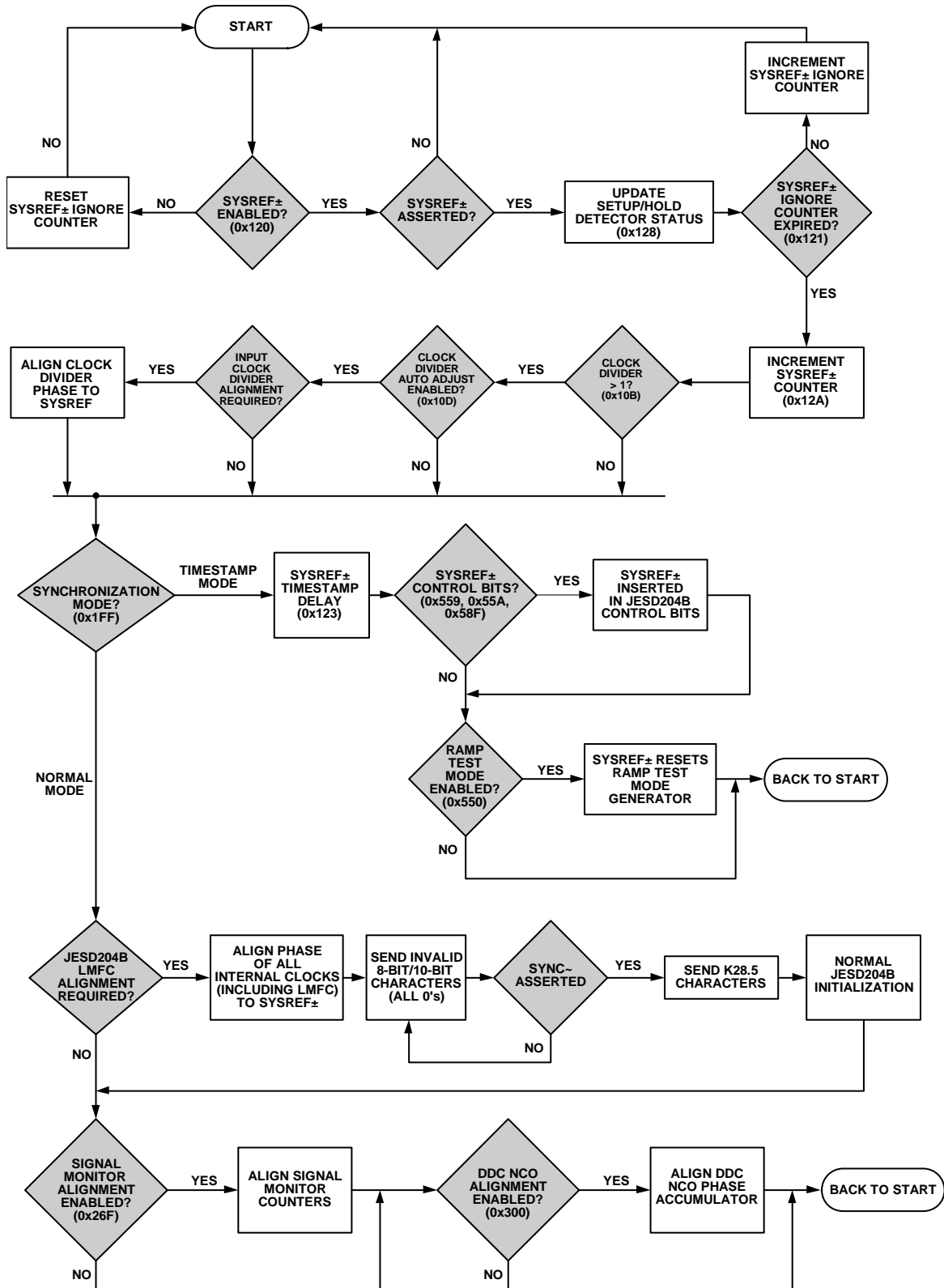
Figure 171. Multichip Synchronization
