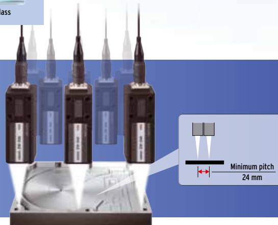
Non-contact Flatness Inspection of HDD Cases
