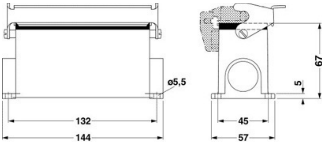
Dimensioned drawing
