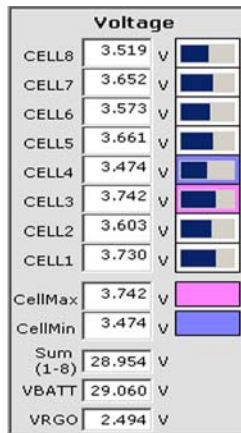
FIGURE 7. VOLTAGE READOUTS
