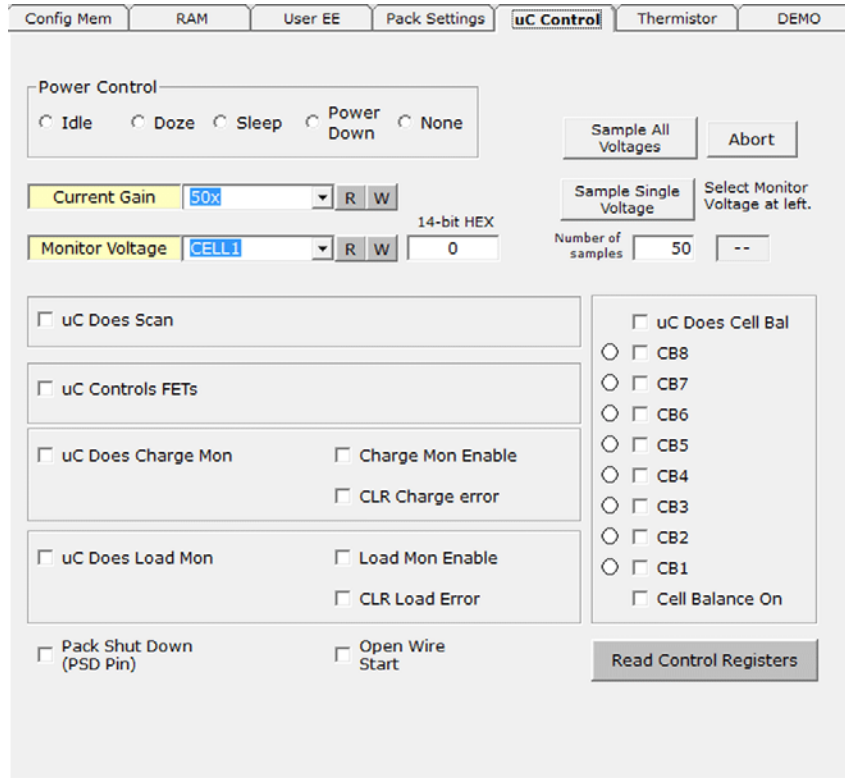
FIGURE 41. ISL94202 GUI - \mu C CONTROL TAB
