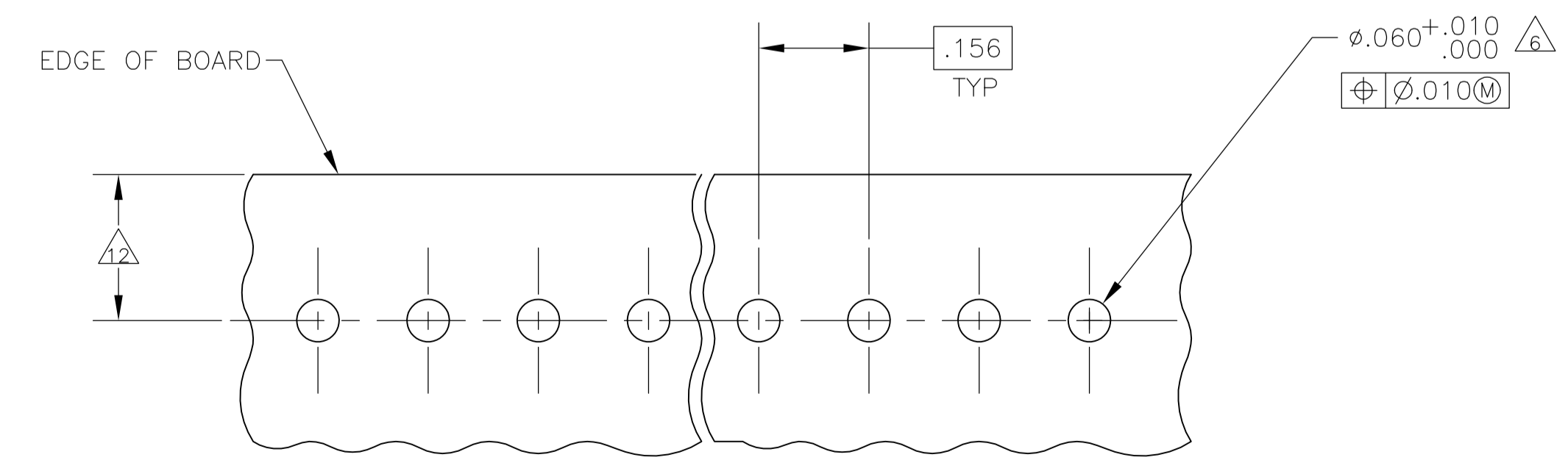
RECOMMENDED MOUNTING HOLE PATTERN (A) FOR .063 THICK P.C. BOARD
