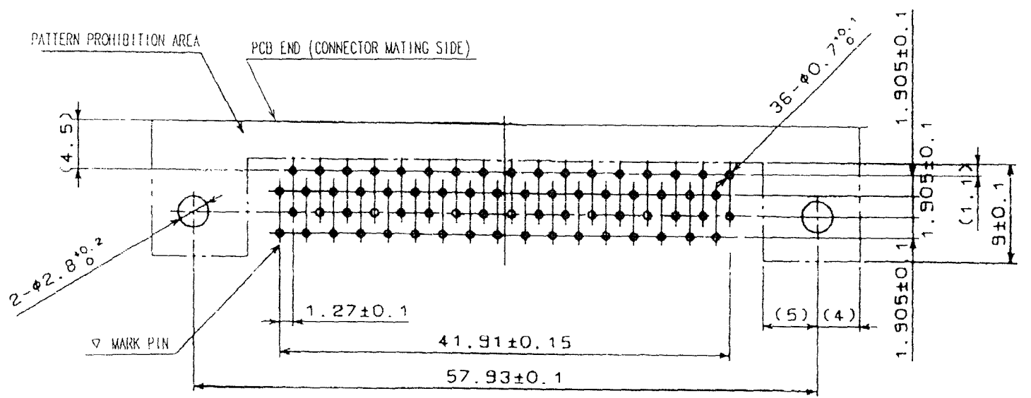
RECOMMENDED PC BOARD PATTERN (RECOMMENDED BOARD THICKNESS 1.6mm)
