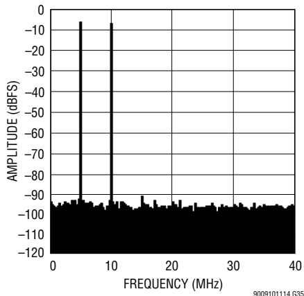
LTM9009-14: 8k Point 2-Tone FFT, f_{IN} = 70\text{MHz} , 75\text{MHz} , -7\text{dBFS} per Tone, 80\text{Mps}
