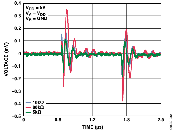
Figure 32. Digital Feedthrough
