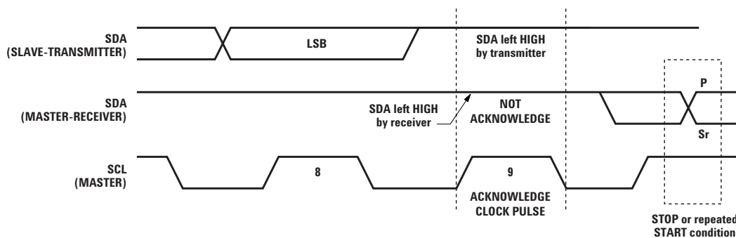
Figure 8. Master-receiver acknowledge
