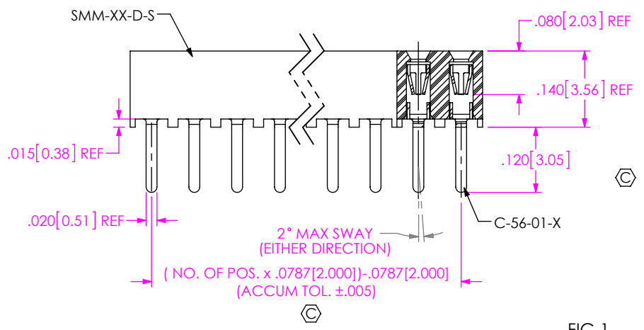
FIG 1 -01: THROUGH HOLE
