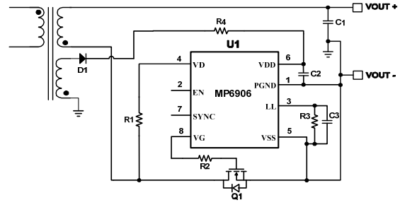
Figure 10: IC Power Derived from the Auxiliary Winding in Low-Side Rectification
