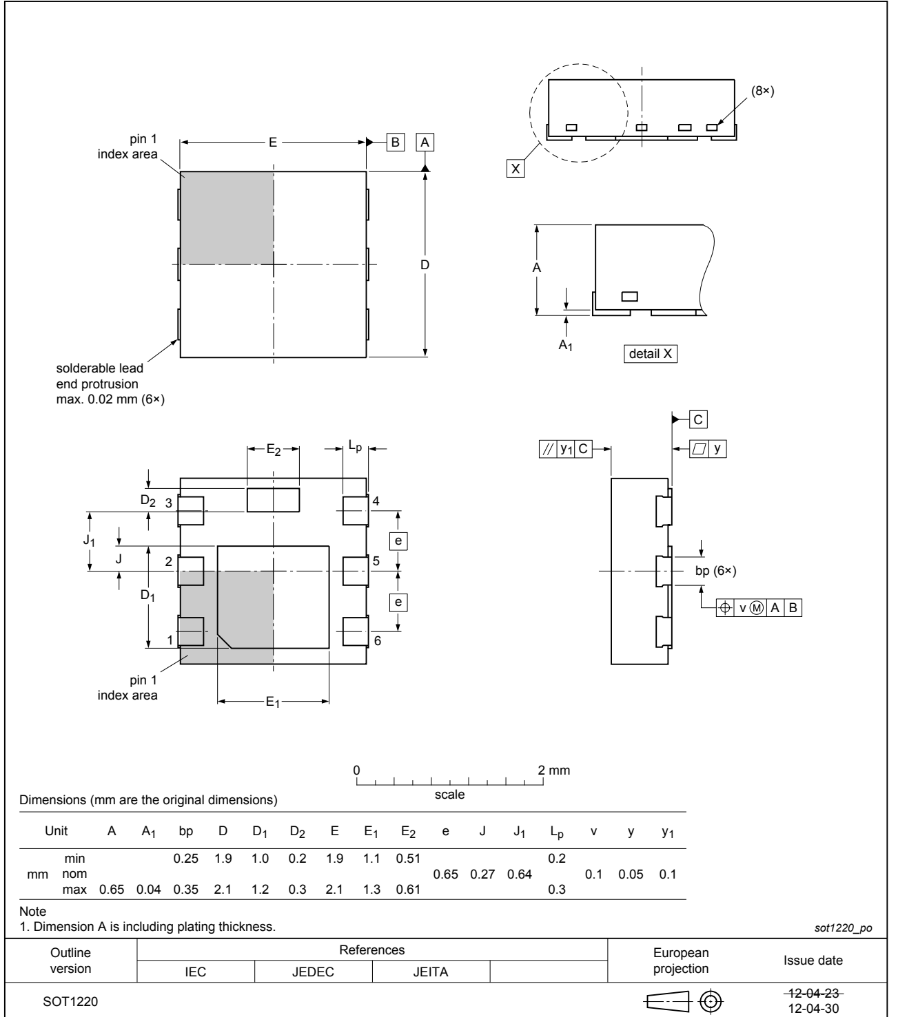
Fig. 17. Package outline DFN2020MD-6 (SOT1220)
