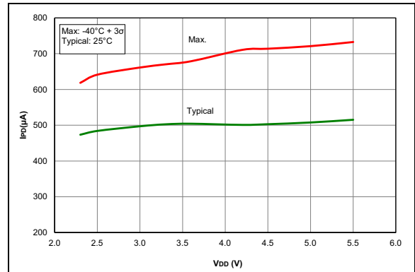
FIGURE 36-36: I_{PD} , Comparator, NP Mode ( CxSP = 1 ), PIC16F1614/8 Only.
