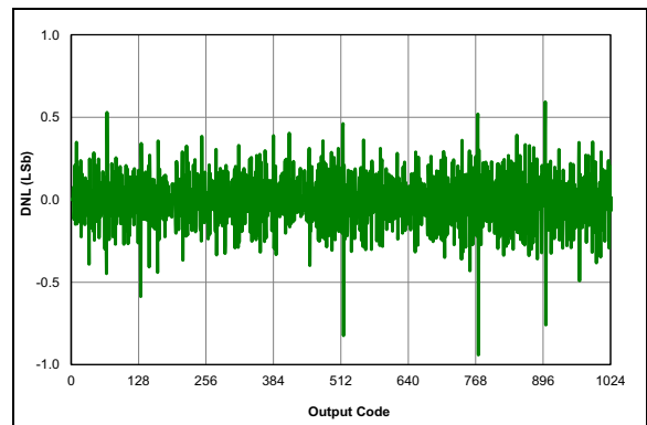
FIGURE 36-66: ADC 10-bit Mode, Single-Ended DNL, V_{DD} = 3.0V , T_{AD} = 4\ \mu\text{s} , 25^\circ\text{C} .
