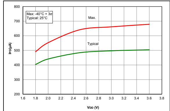
FIGURE 36-35: I_{PD} , Comparator, NP Mode ( CxSP = 1 ), PIC16LF1614/8 Only.
