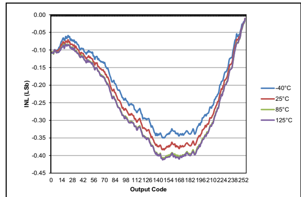
FIGURE 36-95: Typical DAC INL Error, V_{DD} = 5.0V , V_{REF} = \text{External } 5V , PIC16F1614/8 Only.
