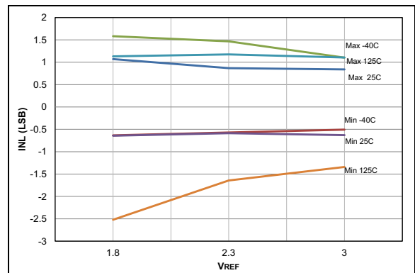
FIGURE 36-72: ADC 10-bit Mode, Single-Ended INL, V_{DD} = 3.0V , T_{AD} = 1\ \mu\text{s} .
