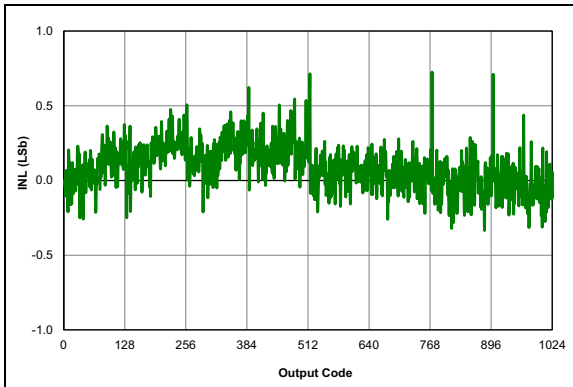
FIGURE 36-67: ADC 10-bit Mode, Single-Ended INL, V_{DD} = 3.0V , T_{AD} = 1\ \mu\text{s} , 25^\circ\text{C} .
