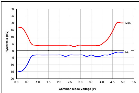
FIGURE 36-86: Comparator Offset, NP Mode ( CxSP = 1 ), V_{DD} = 5.0V , Typical Measured Values at 25^\circ\text{C} , PIC16F1614/8 Only.
