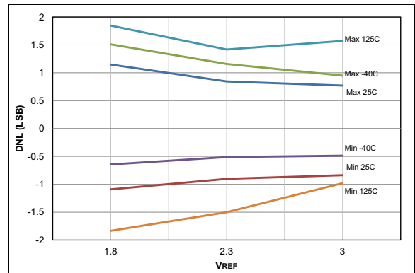
FIGURE 36-71: ADC 10-bit Mode, Single-Ended DNL, V_{DD} = 3.0V , T_{AD} = 1\ \mu\text{s} .
