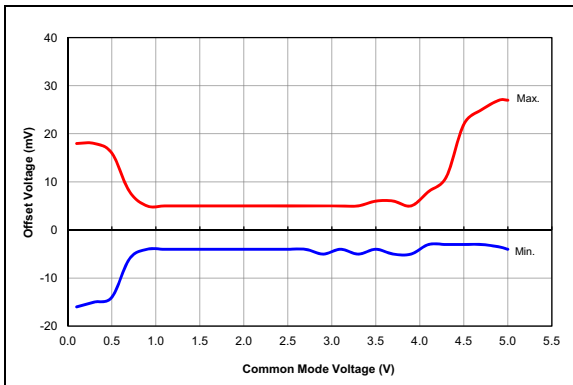
FIGURE 36-87: Comparator Offset, NP Mode ( CxSP = 1 ), V_{DD} = 5.5V , Typical Measured Values From -40^\circ\text{C} to 125^\circ\text{C} , PIC16F1614/8 Only.
