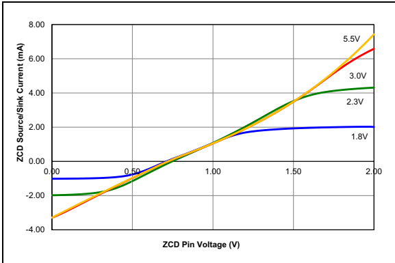
FIGURE 36-103: ZCD Pin Current over ZCD Pin Voltage, Typical Measured Values from -40^\circ C to 125^\circ C .
