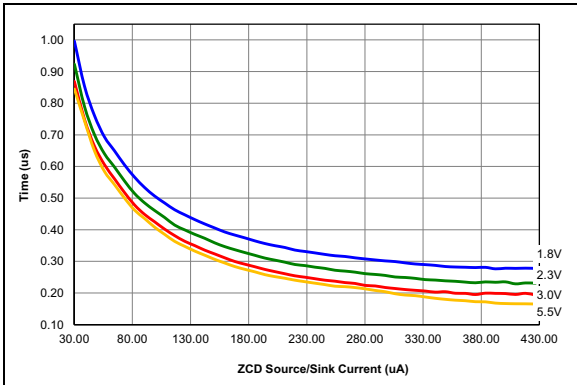
FIGURE 36-104: ZCD Pin Response Time over Current, Typical Measured Values from -40^\circ C to 125^\circ C .
