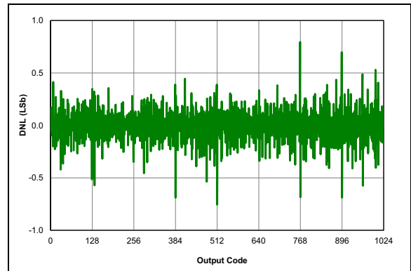
FIGURE 36-65: ADC 10-bit Mode, Single-Ended DNL, V_{DD} = 3.0V , T_{AD} = 1\ \mu\text{s} , 25^\circ\text{C} .
