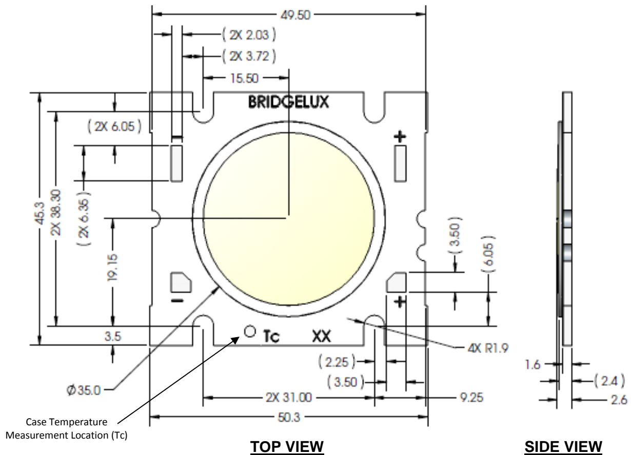
Figure 18: Drawing for RS Part Numbers BXRA-xxH4000-H-03 and BXRA-xxH7000-J-03
