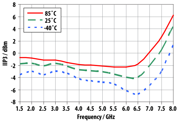
Figure 39. IIP3 vs Frequency
