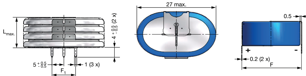
Fig. 12 - Form K: Stacked Through Hole Oval Horizontal
