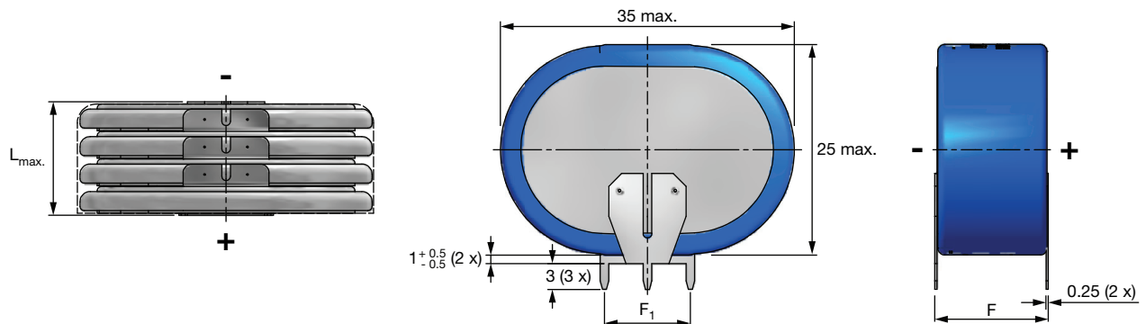
Fig. 13 - Form G: Stacked Through Hole Oval (PCBD)
