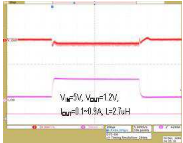
Figure 14. Load Transient
