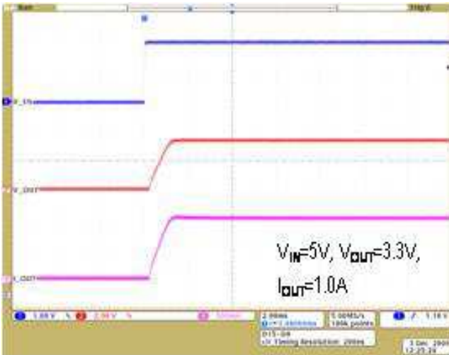
Figure 13. Enable-ON Waveform
