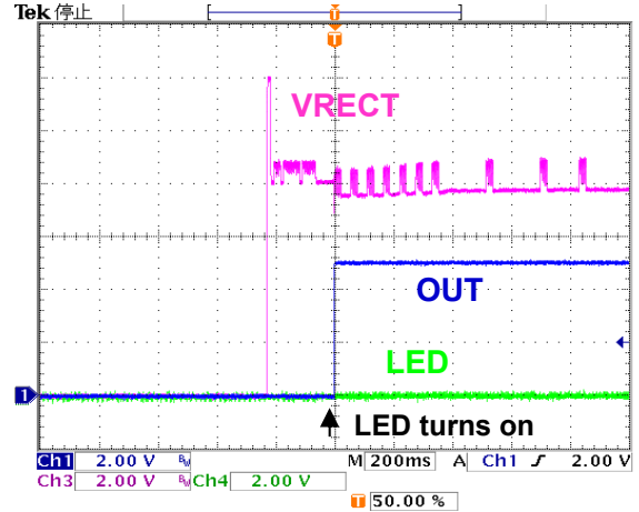
Figure B-18 LED Characteristics 2
