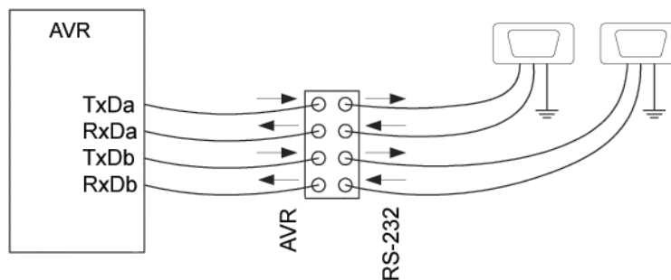
Figure 7-2: RS-232 connection
