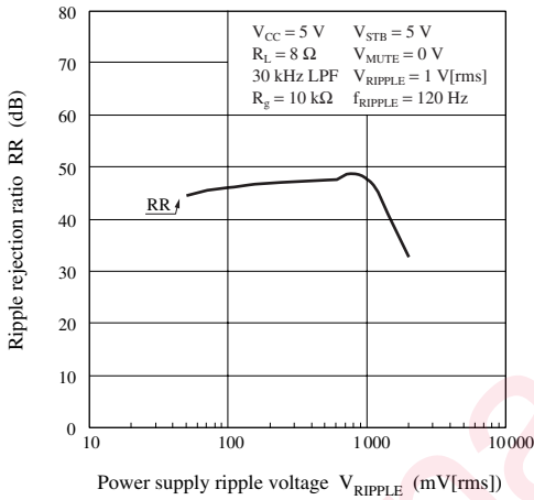
RR — V_{\text{RIPPLE}}
