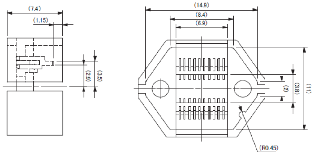
< Bottom view >
