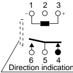
1-coil latching
