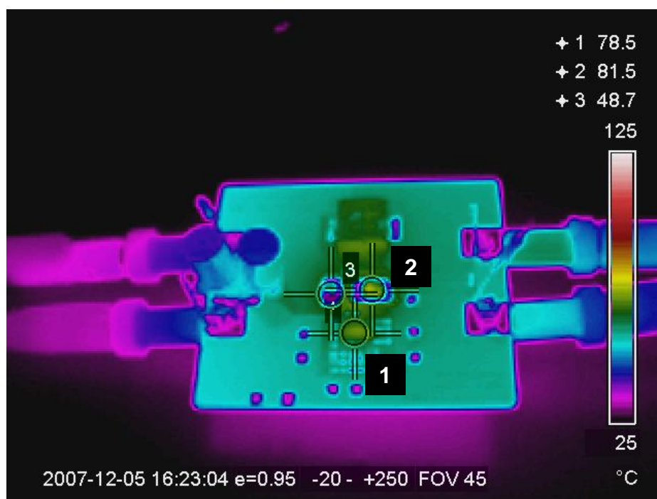
Fig. 12 Thermal Image of IR3629A Demo Board at I o =20A (1: IR3629A, 2: IRF6715, 3: IRF6712)
