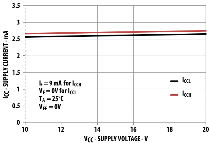
Figure 5 I_{CC} vs. V_{CC}
