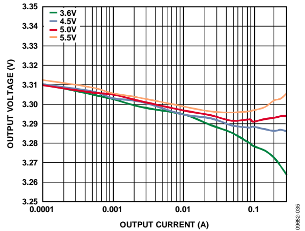
Figure 30. LDO Load Regulation Across Input Voltage, V_{OUT2} = 3.3 V
