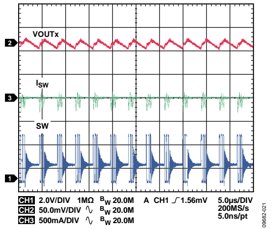
Figure 20. Typical Waveforms, V_{OUT1} = 1.8\text{ V} , I_{OUT1} = 30\text{ mA} , Auto Mode
