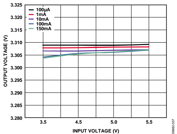
Figure 32. LDO Line Regulation Across Output Load, V_{OUT2} = 3.3 V
