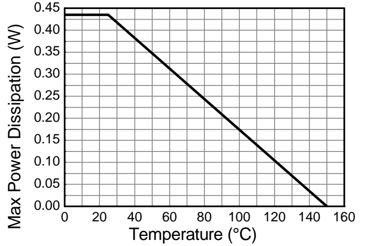
Derating Curve
