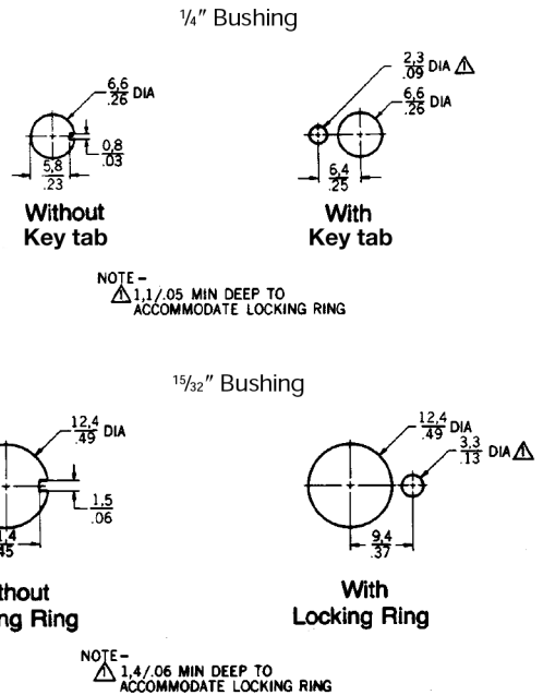
Figure 16. Panel Cutouts
