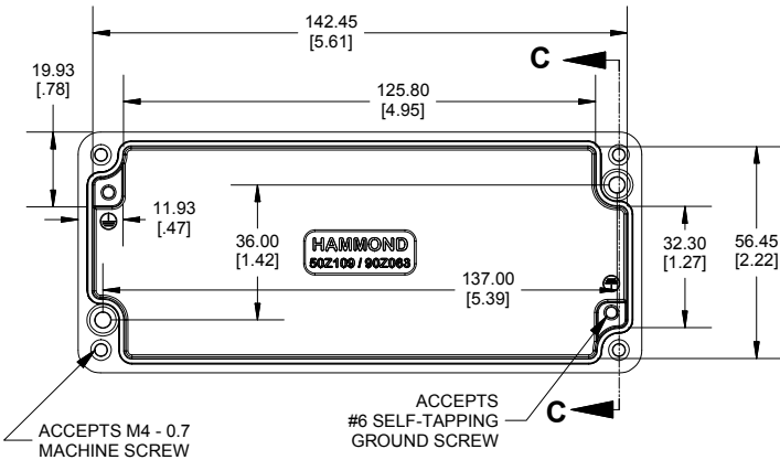
INSIDE BOX
