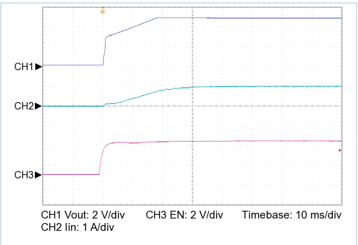
Figure 17 — Startup from EN, V_{IN} = 270\text{ V} , C_{OUT\_EXT} = 10000\ \mu\text{F} , R_{LOAD} = 0.100\ \Omega
