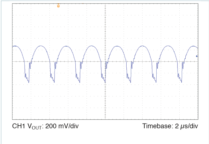
Figure 19 — Output voltage ripple, V_{IN} = 270\text{ V} , V_{OUT} = 5.0\text{ V} , C_{OUT\_EXT} = 1000\ \mu\text{F} , R_{LOAD} = 0.100\ \Omega
