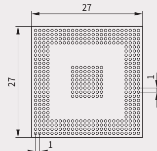
BGA-416
